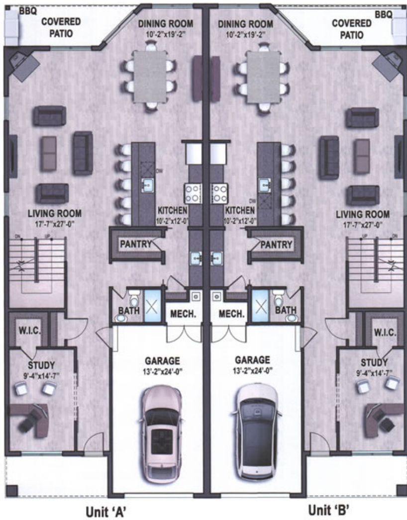
First Floor Plan 1,490 SF
